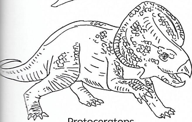
Protoceratops
